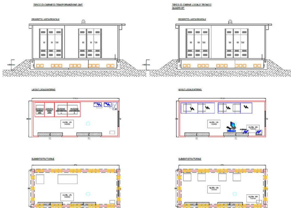
Figura 5.1: Power Station
