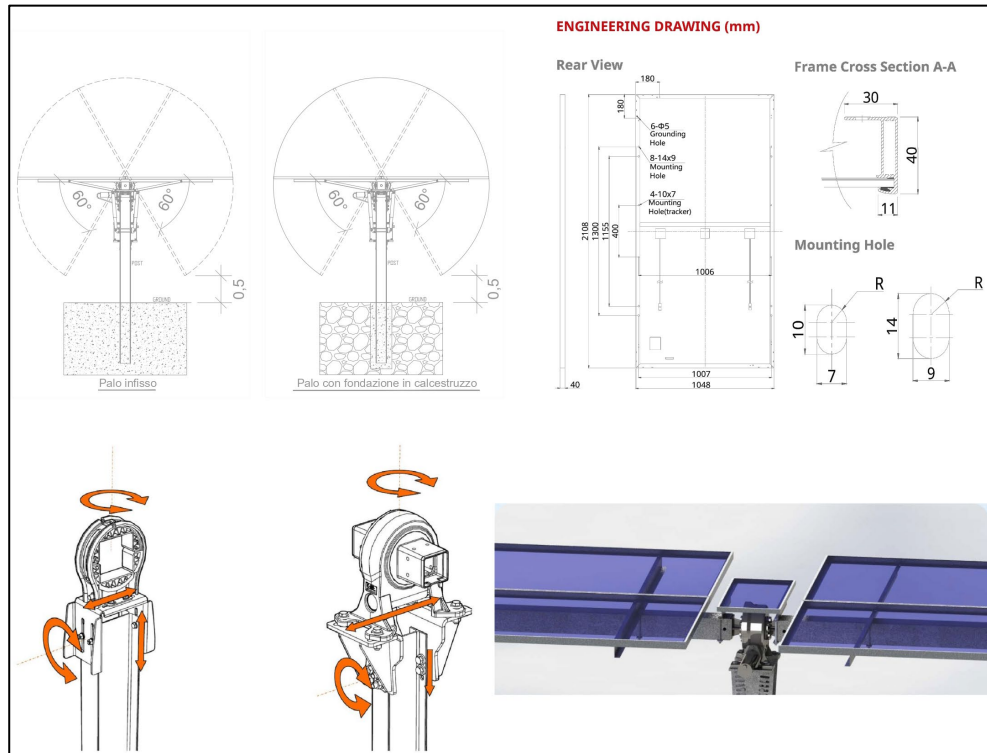
Figura 8.6: Tracker Monoassiale
