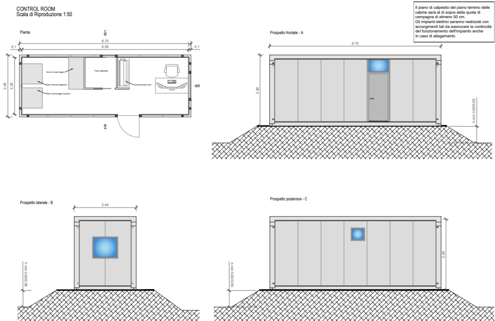
Figura 2.5: Control Room
