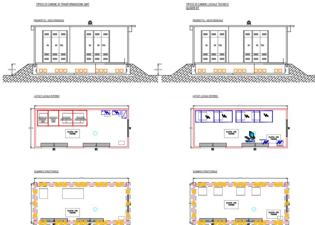
Figura 2.5: Power Station
