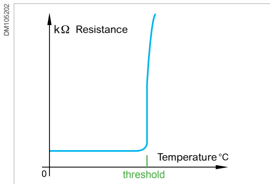
Typical graph of a PTC sensor
